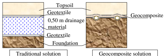
Figure 2. Drainage under embankment
