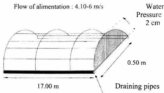
Figure 2. Pressure between the draining pipes.
